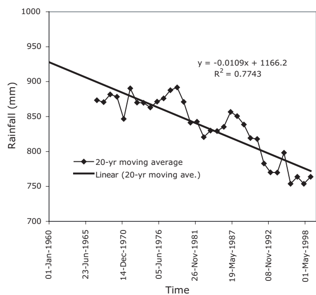
Figure 4. Twenty-year Moving Average of Precipitation in Gwembe Valley.
